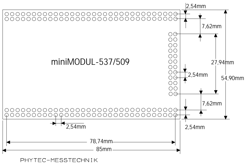
Figure 13: Physical Dimensions
