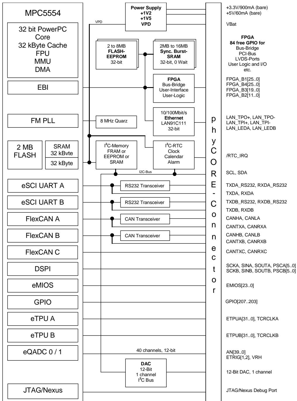
Figure 1: Block Diagram phyCORE-MPC5554
