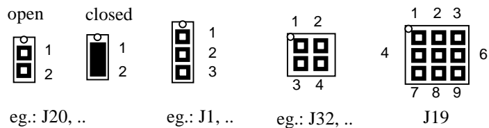
Figure 5: Numbering of the Jumper Pads
