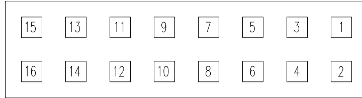
Fig. 29-3. UART3/UART2 Header Connector X13 Pin Numbering
