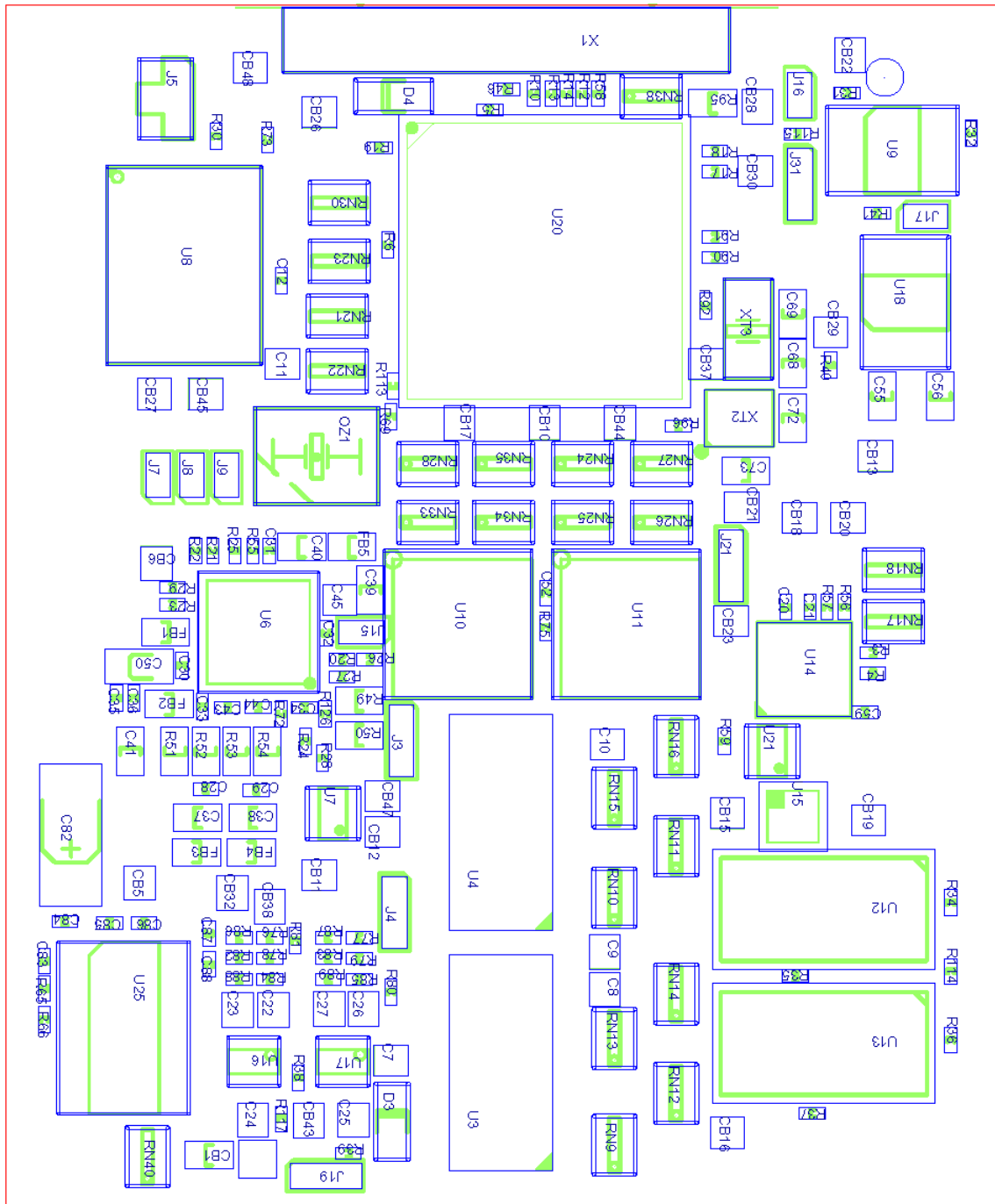
Fig. 1-2. Top View of the phyCORE-LPC3250 (Controller Side)
